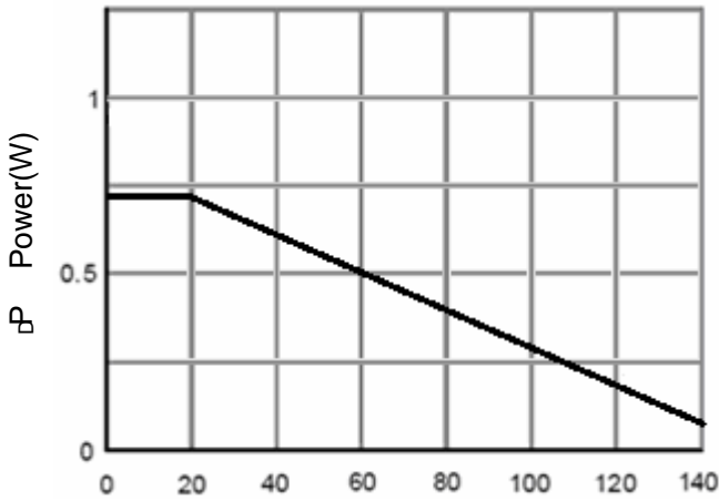
Figure 1 Power Dissipation
