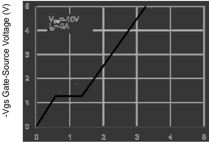
Figure 9 Gate Charge
